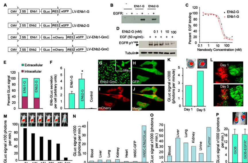
Fig. 2. Pharmacokinetics of anti-EGFR nanobodies in vitro and in vivo. (A) Schematic representation of lentiviral transfer vectors bearing imageable anti-EGFR nanobodies (ENb1 and ENb2) genetically fused to Gaussia luciferase (GLuc) or to a fusion of GLuc and mCherry. (B) Western blot analysis showing the EGFR specificity of GLuc nanobody variants on EGFR-negative [NIH 3T3 (-)] and EGFR-positive [Her14 (+)] cell lines incubated with or without ENb-GLuc. (C) ELISA showing the EGF competition by anti-EGFR ENb-GLuc variants. (D) Western blot analysis showing inhibition of EGFR activation by nanobody-GLuc variants on serum-starved Her14 cells incubated with serial dilutions of ENb2-G. (E) Gluc bioluminescence assay showing the presence of nanobody-GLuc fusion proteins intracellularly and in the culture medium in human NSC expressing ENb1-G and ENb2-G. (F) Dual bioluminescence assay on human NSC coexpressing GFP-FLuc and ENb1-G or ENb2-G showing the ratio of nanobody-GLuc fusion in the culture medium and the relative cell number by measurement of GLuc and FLuc activity, respectively. (G–J) Fluorescence confocal microscopy on hNSC expressing ENb2-GmC showing the intracellular localization of nanobodies (red) and GFP (green). (K and L) Combined intravital microscopy and bioluminescence imaging of U87-FLuc-TdTomato GBM (red)-bearing SCID mice implanted s.c. with human NSC expressing ENb2-G (green) in a dorsal skinfold window chamber. Mice were imaged on day 1 and 5 after NSC implantation by bioluminescence imaging for the secretion of ENb2-G (K) and by intravital microscopy for the fate of NSC (L). (M) In vivo bioluminescence imaging of purified ENb2-G injected into mice bearing established Gli36-Fluc-mCherry tumors by i.v. injection and analyzed at different time points after coelenterazine injection. (N) Ex vivo analysis of biodistribution of NSC-delivered ENb2-G assessed by GLuc imaging of organs. (O) Ex vivo analysis of biodistribution of systemically administered purified ENb2-G assessed by GLuc imaging of organs. (P) Mice bearing Gli36-Fluc-mCherry (left flank) and the EGFR overexpressing Gli36-Fluc-mCherry-EGFR + (right flank) s.c. tumors were given purified ENb2-G protein i.v. and were imaged for GLuc. Representative image and summary graph showing localization of ENb2-G in mice. In all graphs, error bars represent SEM. Data were represented as mean \pm SEM, and * denotes P < 0.05 , Student's t test.
