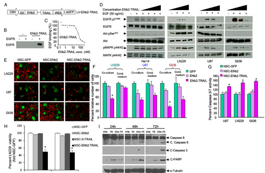
Fig. 3. Efficacy of the dual effector molecule ENb2/TRAIL. (A) Schematic representation of lentiviral transfer vectors bearing cytotoxic variant of EGFR nanobody, ENb2-TRAIL. (B) Western blot analysis showing the EGFR specificity of ENb2-TRAIL on NIH 3T3 and Her14 cell lines incubated with or without ENb2-TRAIL. (C) ELISA showing the EGF competition by ENb2-TRAIL. (D) Western blot analysis showing inhibition of EGFR and downstream signaling via the AKT and MAPK pathways on serum-starved Her14 and GBM (LN229, U87, Gli36) cells incubated with ENb2-TRAIL. (E) Fluorescence microscopy on Fluc-mCherry expressing GBM cells (LN229, U87, and Gli36) cocultured with mouse NSC expressing GFP (control), ENb2, or ENb2-TRAIL. (F) Relative GBM cell viability in coculture or after incubation with conditioned medium from mNSC expressing GFP, ENb2, or ENb2-TRAIL for 72 h as determined by measuring Fluc activity. (G) Caspase 3/7 activity in coculture of GBM cells and mNSC. (H) Relative LN229-mCherry-Fluc cell viability in coculture with mNSC expressing GFP, ENb2, S-TRAIL, or ENb2-TRAIL for 72 h as determined by measuring Fluc activity. (I) Western blot analysis of LN229 cells treated with mNSC expressing ENb2, S-TRAIL, or ENb2-TRAIL. Data were represented as mean \pm SEM and * denotes P < 0.05 , Student's t test.
